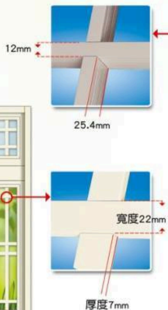
門用格子窗
